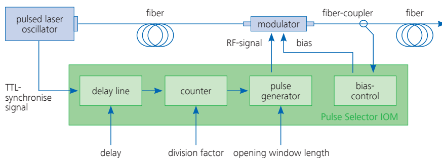
Application scheme
